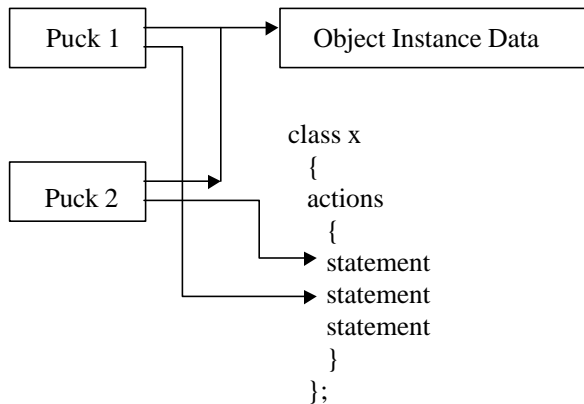
Figure 5: An Active Object With Two Pucks
