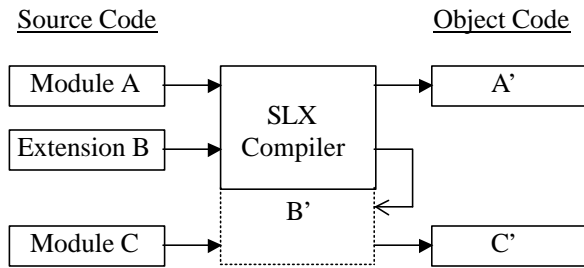
Figure 3: SLX Compiler Architecture
